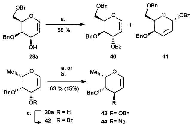
Scheme 5 Reagents, conditions (and yields): (a) PPh 3 , BzOH, DEAD, toluene, 20 h, 0 °C→rt, 58% from 28a and 63% from 30a ; (b) LiN 3 , PPh 3 , CBr 4 , DMF, rt, 12 h, 15% from 30a ; (c) BzCl, pyr, CH 2 Cl 2 , 12 h, rt, 30%.
